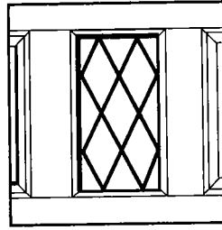
Tudor I Glazing Detail (Cast Aluminum)
